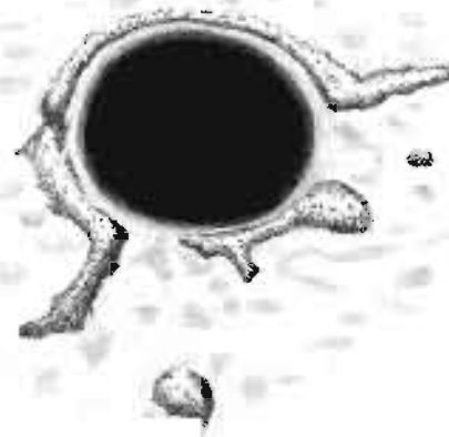
Great Blue Hole, Belize underwater sinkhole, caused by seismic movement ocean system
