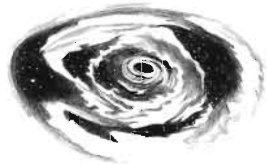
PKS 1127-145 supermassive blackhole in the heart of a quasar
