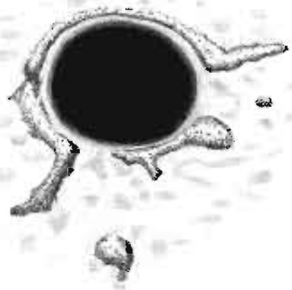
Great Blue Hole, Belize underwater sinkhole caused by collapse limestone cave system
